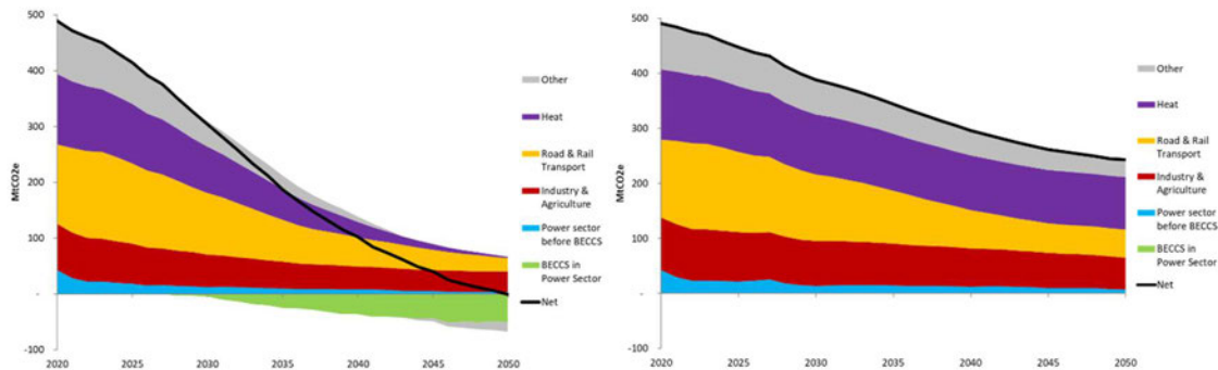
Figure 7-1: NGENSO scenarios, showing the importance of a whole-society approach to decarbonisation and low carbon electricity generation. [104, Data sheet, Figures NZ.5]
