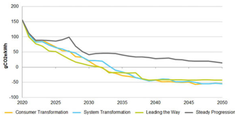
Figure 5-2: Power generation emissions must reduce to negative in the early 2030s to meet the 2050 Net Zero target [104, Figure SV.27]
