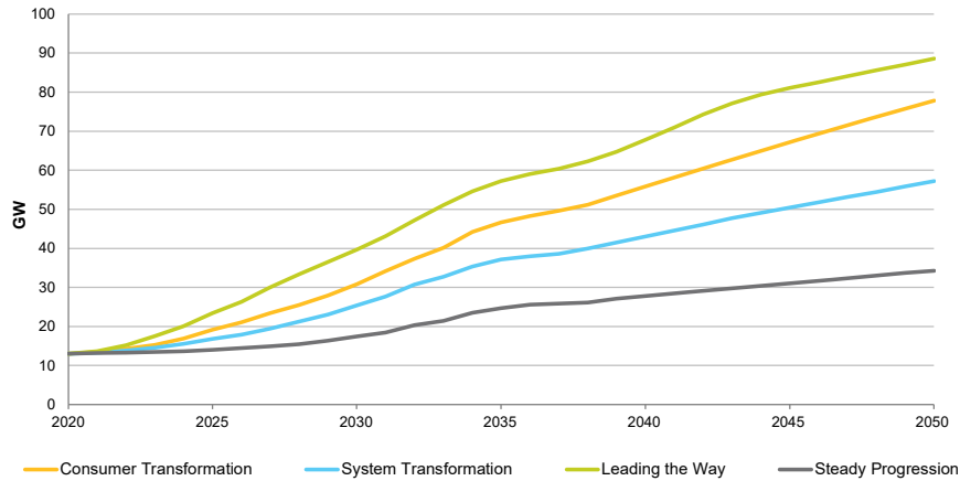
Figure 5-1: Illustration of potential solar capacity evolution by FES scenario [104, Figure SV.31]
