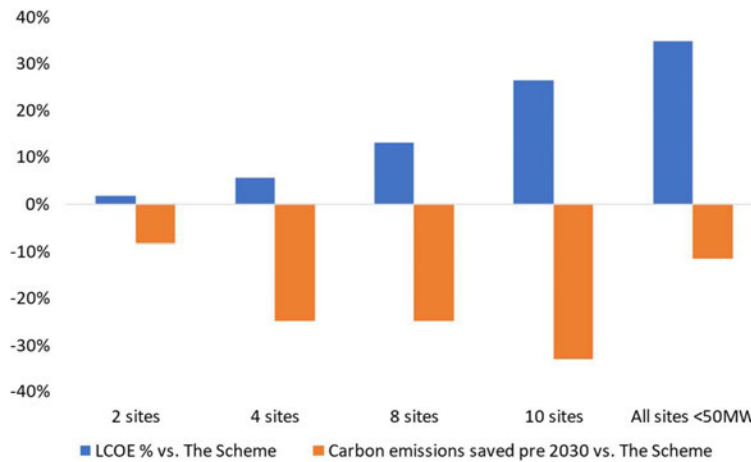
Figure 11-6: LCOE and carbon emissions savings at large-scale single-site solar, versus developing the same total capacity across multiple projects [Author analysis]
