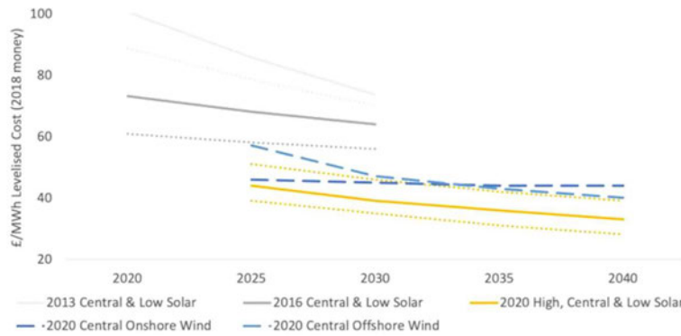
Figure 11-5: BEIS Cost of Generation. An evolution of Levelised Cost forecasts [14, and Author analysis]
