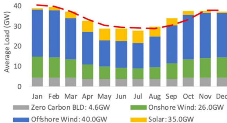
Figure 9-3: Deploying 35GW of large-scale solar alongside government offshore wind ambitions (40GW) meets anticipated seasonal demand levels [7, Market data, Author analysis]
