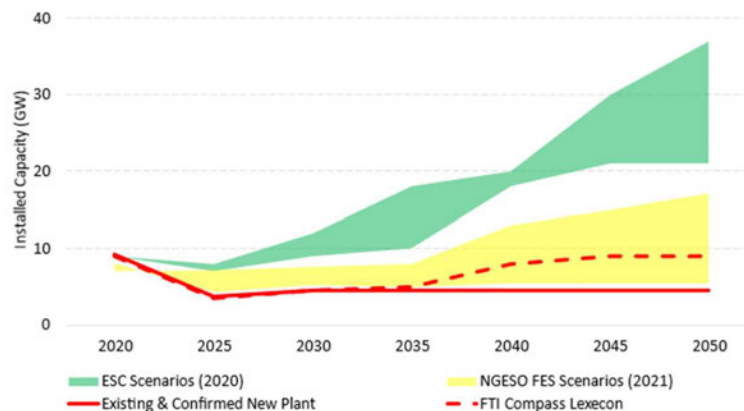
Figure 5-4: Projections of current nuclear capacity as existing stations close. Source: [7, 8, 9, Author Analysis, www.edfenergy.com ]
