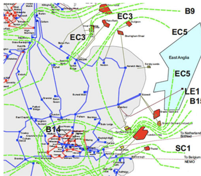
Figure 10-1: The NETS in the vicinity of Bulls Lodge [10, Appendix A]
