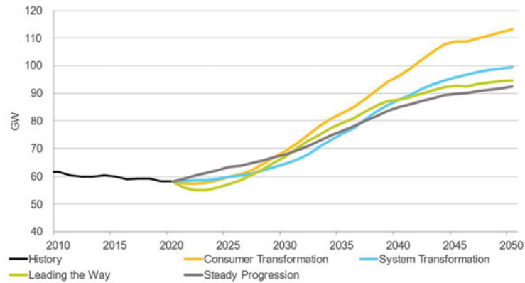
Figure 7-2: Future net peak electricity demand [104, Figure FL.4]
