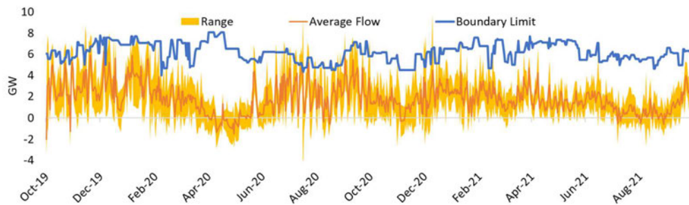
Figure 10-2: Day ahead constraint limit and flow into the south east of England [11, Author Analysis]
