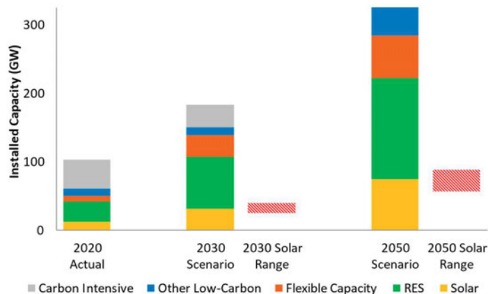
Figure 8-1: Generation capacity by technology type and amount of renewable capacity for 2030 and 2050 [104, Figure SV.22]
