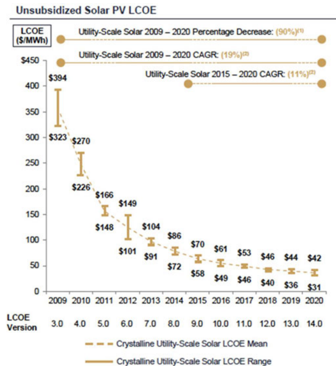
Figure 11-4: Historical reductions in the LCOE of solar generation [13, p9]
