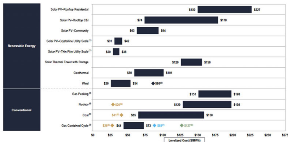
Figure 11-3: Unsubsidised levelised cost of energy comparison [13, p2]
